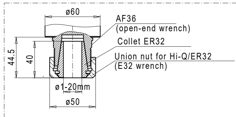
Collet chuck HI-Q/ER32
